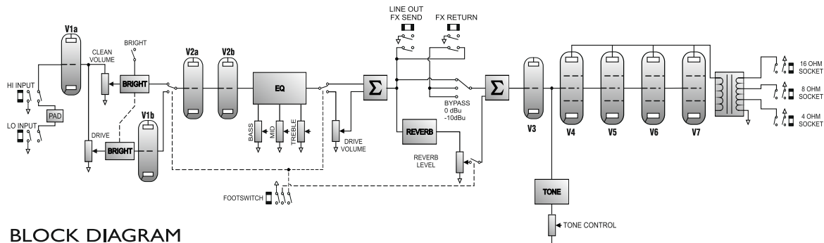
BLOCK DIAGRAM
